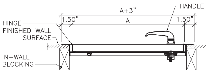
Section Detail
