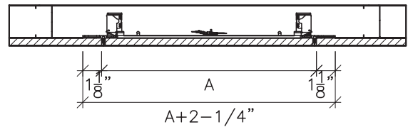
Section Detail
