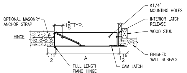
Section Detail
