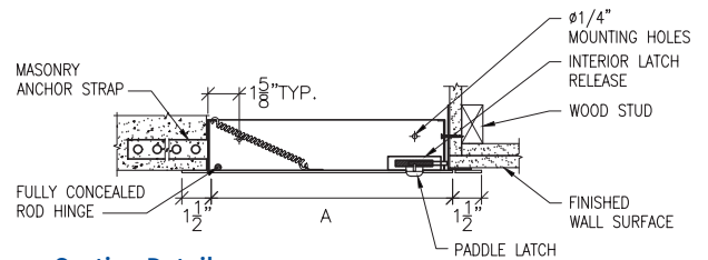
Section Detail
