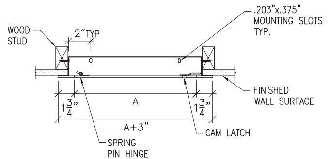
Section Detail
