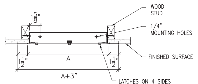
Section Detail
